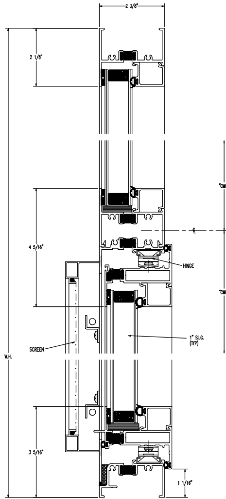
3 OPERATING SILL
