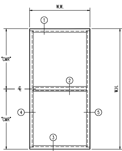
WINDOW ELEVATION (EXTERIOR VIEW)
