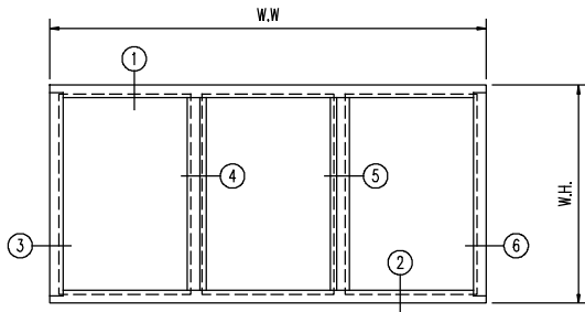
WINDOW ELEVATION (EXTERIOR VIEW)
